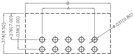
Recommended P.C.Board Layout General Tolerances: ±0.05
